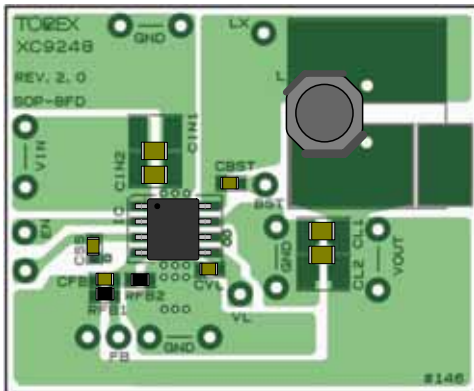
PCB mounted
