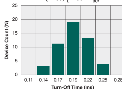
Typical Turn-Off Time (N=50, I_L=100\text{mA}_{DC} )
