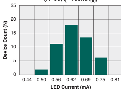
Typical I_F for Switch Dropout (N=50, I_L=100\text{mA}_{DC} )
