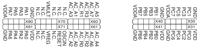
Figure 3 : XE8000EV101 connectors
