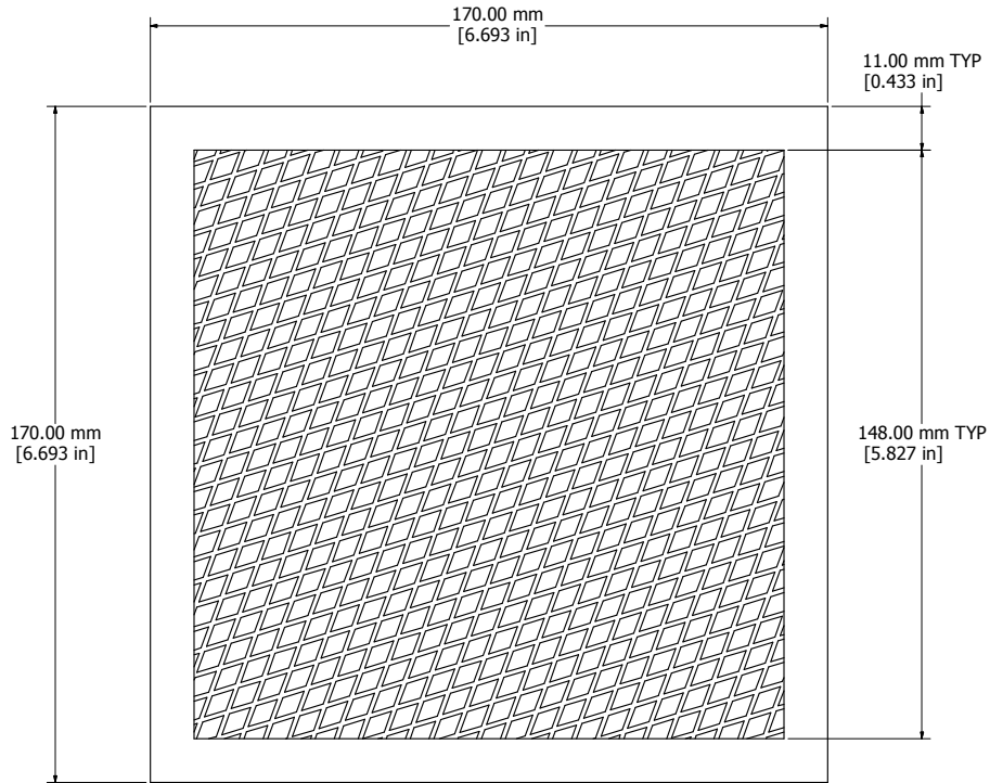
FRONT VIEW
