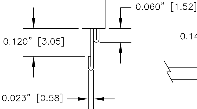
WIRE ATTACHMENT
