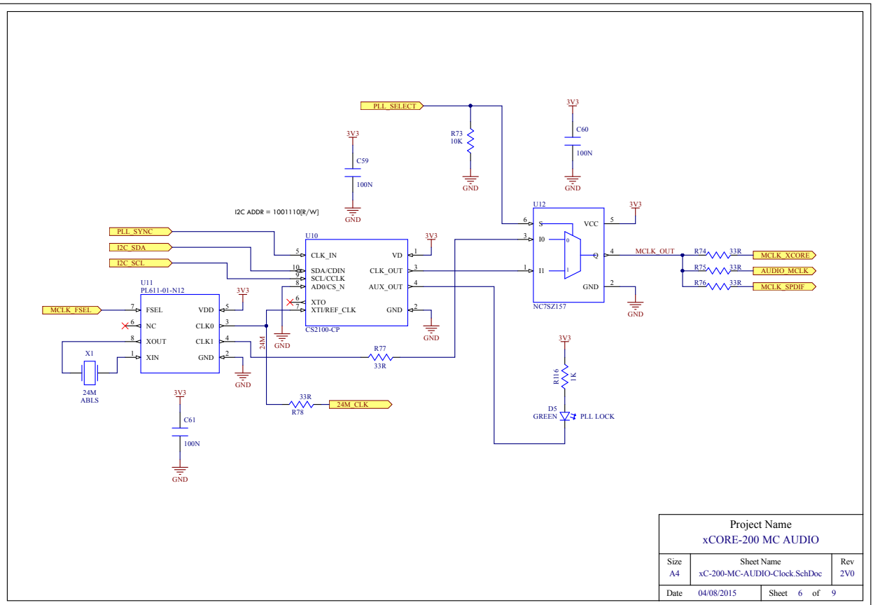
Figure 33: xCORE-200 Multichannel Audio Platform schematic (6 of 9)
