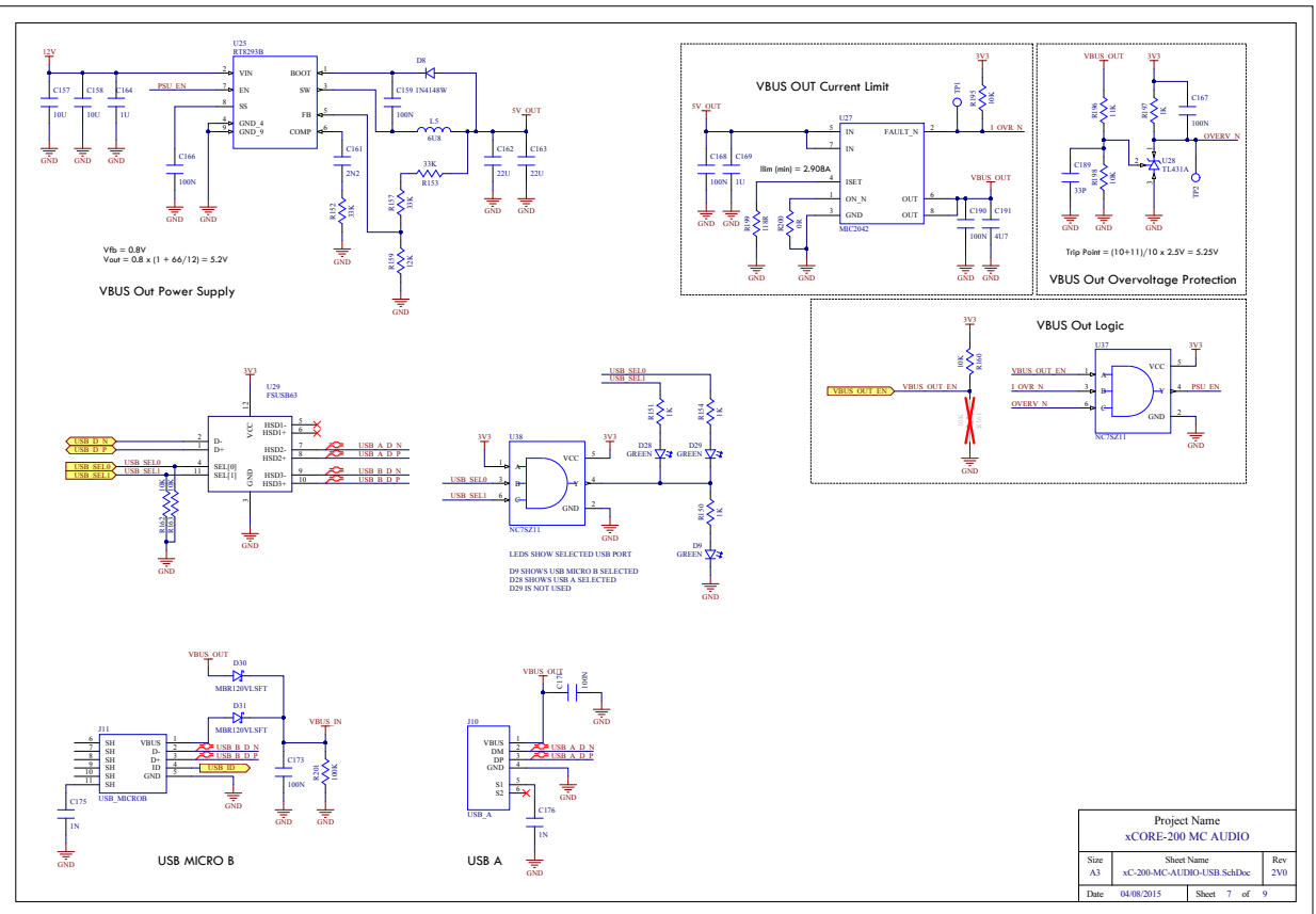
Figure 34: xCORE-200 Multichannel Audio Platform schematic (7 of 9)
