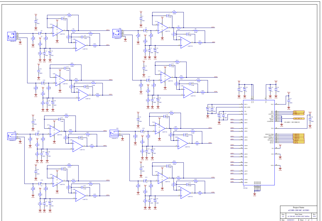
Figure 32: xCORE-200 Multichannel Audio Platform schematic (5 of 9)
