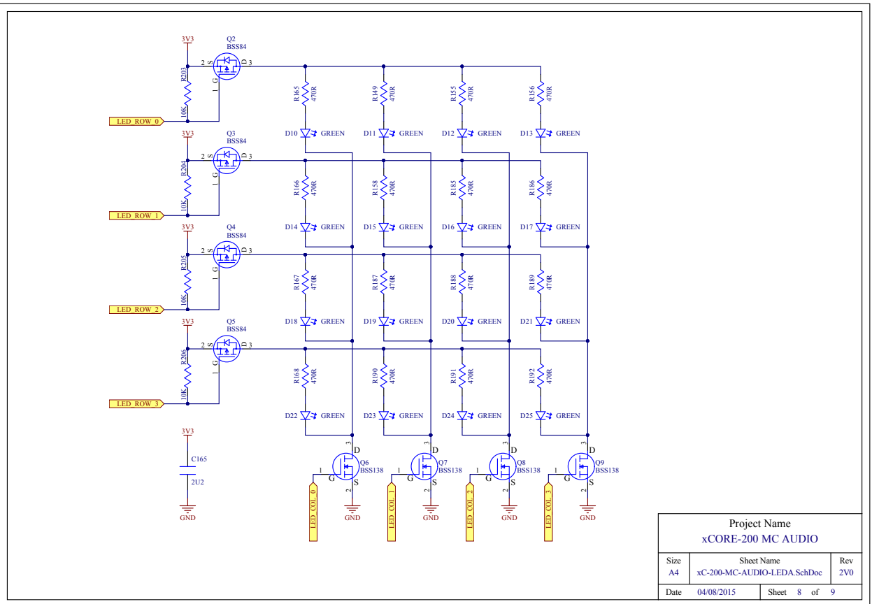
Figure 35: xCORE-200 Multichannel Audio Platform schematic (8 of 9)
