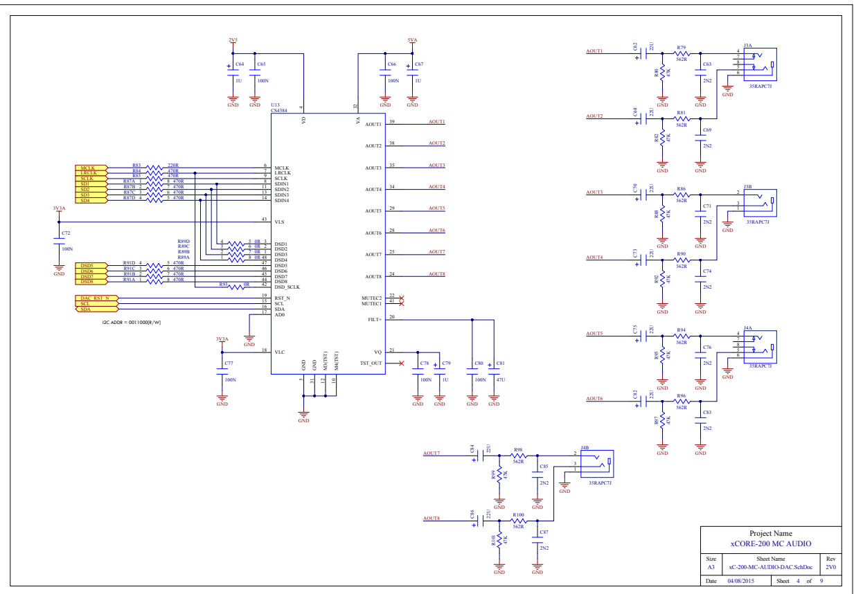
Figure 31: xCORE-200 Multichannel Audio Platform schematic (4 of 9)
