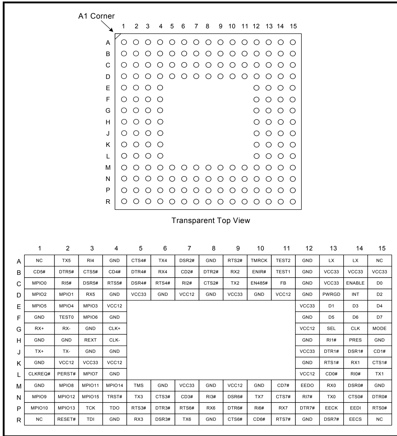
FIGURE 2. 176-FPBGA PINOUT
