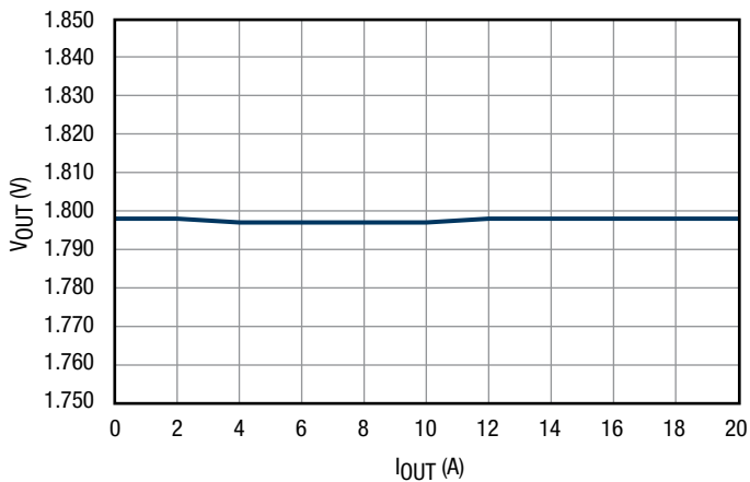
Figure 17. Load Regulation
