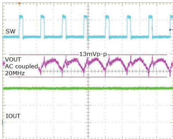
Figure 7. Steady State, I_{OUT} = 20A
