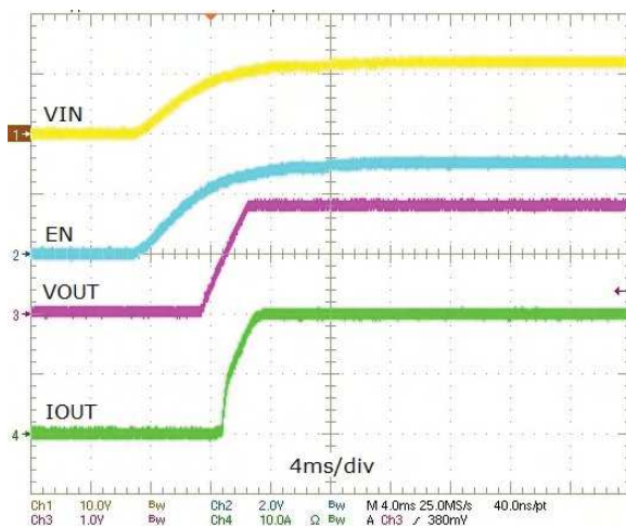
Figure 9. Power-Up, I_{OUT} = 20A
