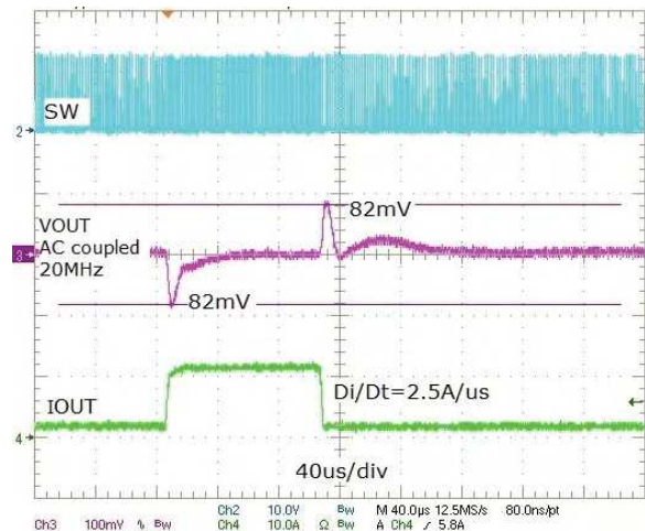
Figure 12. Load Transient, DCM, 1.8A-11.8A-1.8A
