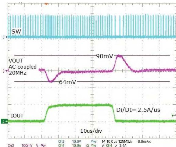
Figure 11. Load Transient, Forced CCM, 0A-10A-0A
