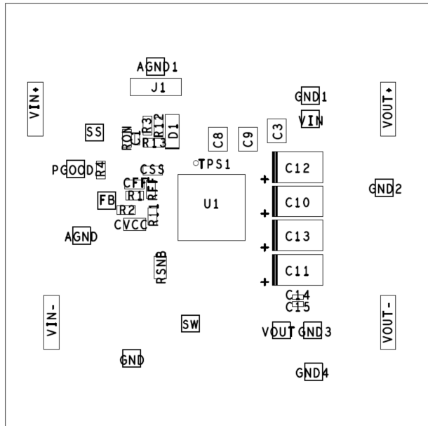
Fig. 3: Assembly Top
