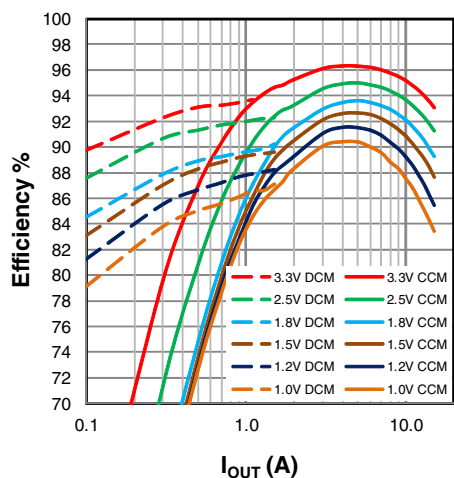
Figure 19: Efficiency, V_{IN}=5\text{V}
