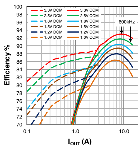
Figure 21: Efficiency, V_{IN}=12\text{V}
