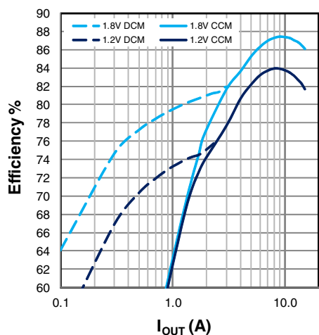
Figure 23: Efficiency, V_{IN}=19.6\text{V}
