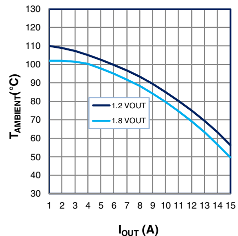
Figure 24: Maximum T_{AMBIENT} vs I_{OUT} , V_{IN}=19.6\text{V}
