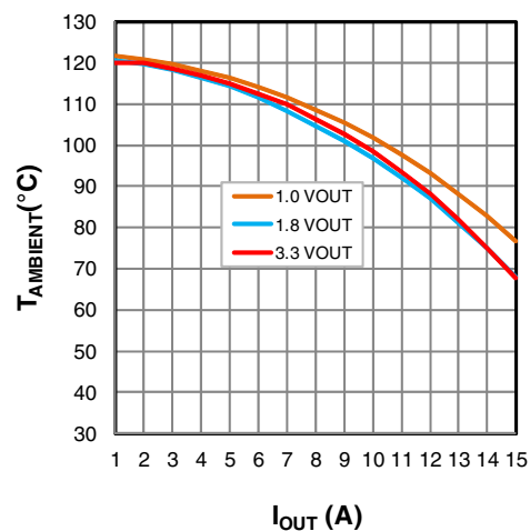
Figure 20: Maximum T_{AMBIENT} vs I_{OUT} , V_{IN}=5\text{V}
