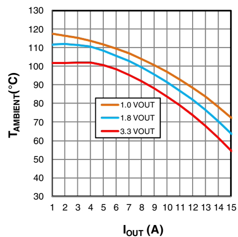
Figure 22: Maximum T_{AMBIENT} vs I_{OUT} , V_{IN}=12\text{V}
