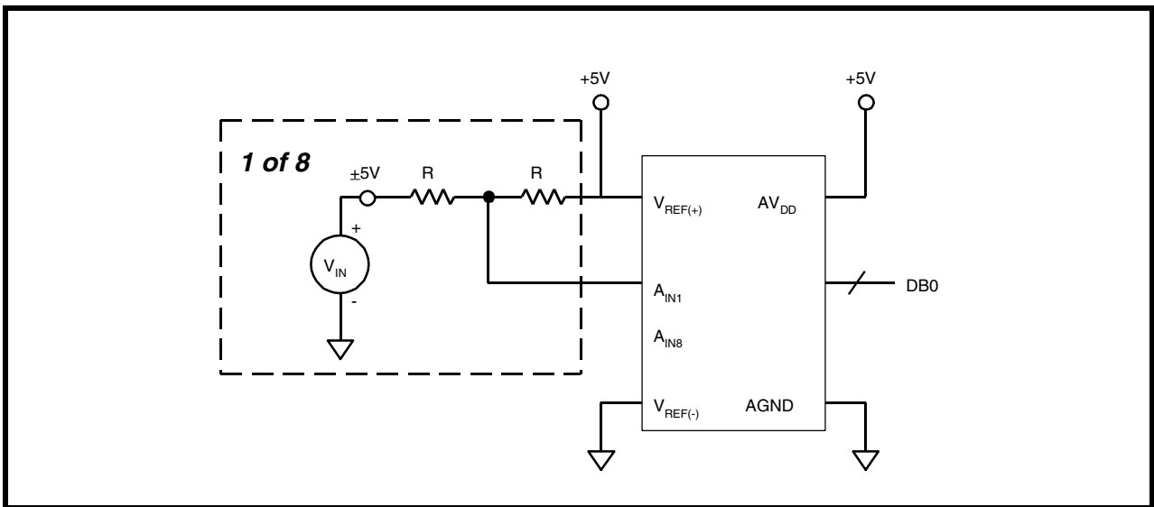
FIGURE 18. ±5V ANALOG INPUT
