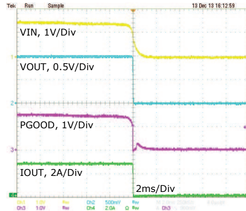
Fig. 10: Powerdown, IOU=3A, 1.5VIN, 1VOUT
