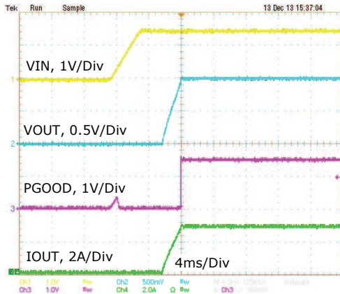
Fig. 9: Powerup, IOU=3A, 1.5VIN, 1VOUT
