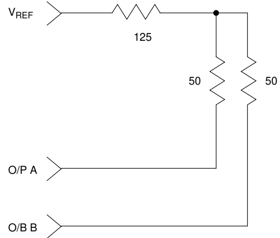
Figure 6. External Transmit Network
