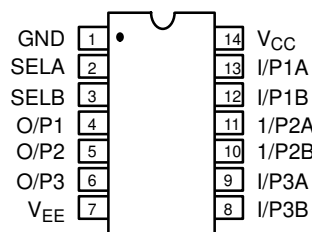
14 Lead CDIP (0.300'') XR-T3589
