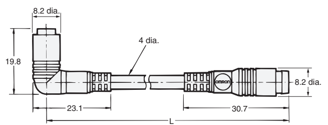
Right-angle/Straight Connectors XS3W-S424-4□□-R
