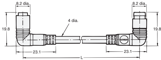
Right-angle/Right-angle Connectors XS3W-S422-4□□-R
