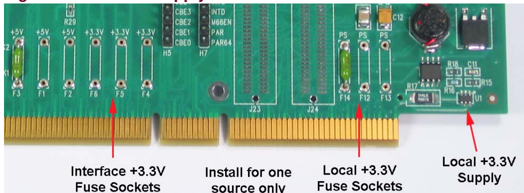
Figure 2.6.1: +3.3 V Supply
