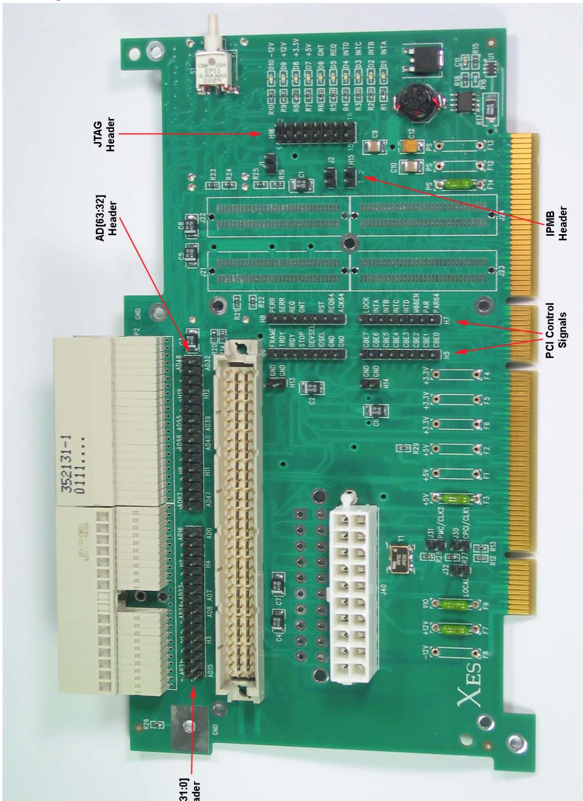
Figure 2.3.4: Header Locations
