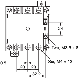
Mounting holes
