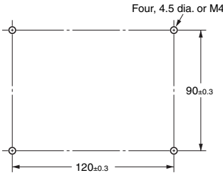
Mounting Holes
