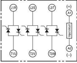
G3PB-445B-3-VD
