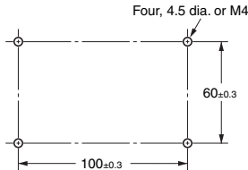
Mounting Holes
