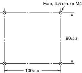
Mounting Holes
