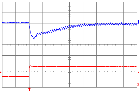
Fig. 1.2V.7: Output voltage response for V_{out} = 1.2\text{ V} to positive load current step change from 10 A to 20 A with slew rate of 5\text{ A}/\mu\text{s} at V_{in} = 5\text{ V} . Top trace: output voltage (100 mV/div.); Bottom trace: load current (10 A/div.). C_o = 100\text{ }\mu\text{F} ceramic. Time scale: 20 \mu\text{s} /div.
