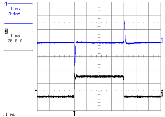
Figure 12. Transient Response to Dynamic Load Change from 0% to 50% of full load ( V_{in} = 12\text{V} , V_o = 1.5\text{V} ). Ch1 – Vout, Ch3 – Iout
