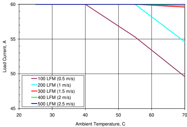
Figure 14. Derating Output Current versus Local Ambient Temperature and Airflow (Vin=12.0V, Vo=1.2V).
