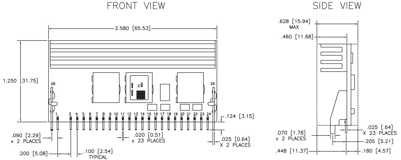
Figure 11. Mechanical Drawing
