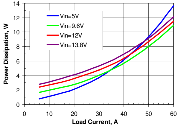
Figure 8. Power Dissipation vs. Load. Vout=1.5V
