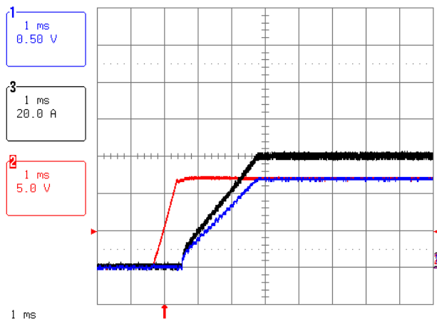
Figure 11. Typical Start-Up with application of V_{in} ( V_o = 1.2\text{Vdc} , I_o = 60\text{A} ). Ch1 – Vout, Ch2 – V_{in} , Ch3 - Iout
