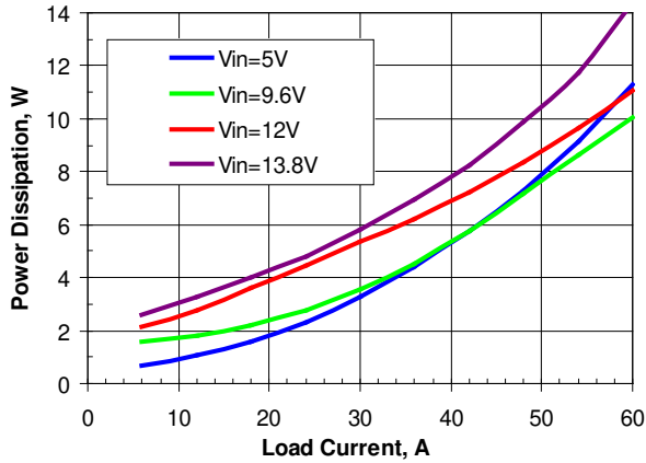
Figure 6. Power Dissipation vs. Load. Vout=0.6V
