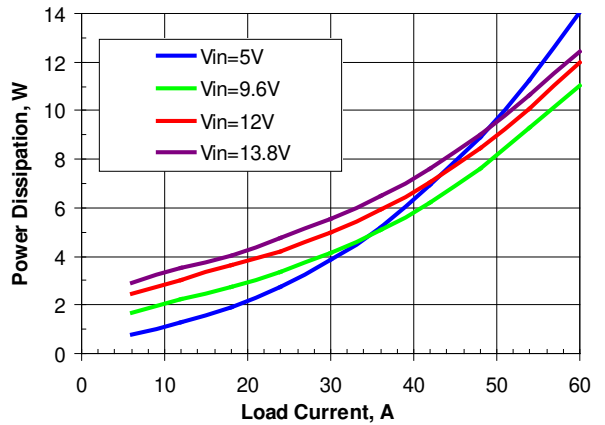
Figure 9. Power Dissipation vs. Load. Vout=1.8V
