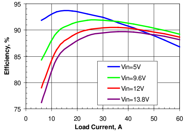
Figure 4. Efficiency vs. Load. Vout=1.5V
