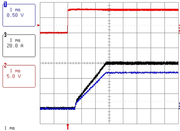
Figure 10. Typical Start-Up Using Remote On/Off ( V_o = 1.2\text{Vdc} , I_o = 60\text{A} ). Ch1 – Vout, Ch2 – On/Off, Ch3 - Iout
