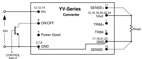
Figure 18. Circuit Configuration For ON/OFF Function
