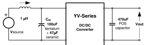
Figure 20. Test Setup For Measuring Input Reflected-Ripple Current And Output Voltage Ripple
