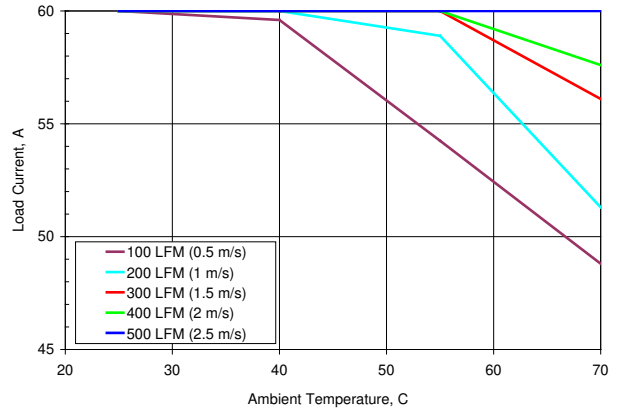
Figure 15. Derating Output Current versus Local Ambient Temperature and Airflow (Vin=12.0V, Vo=1.5V).
