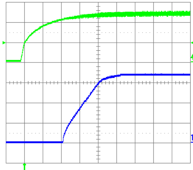
Fig. 19: Turn-on transient for V_{out} = 3.3\text{ V} with the application of the input voltage at full rated load current (resistive) and 1\ \mu\text{F} external capacitance at V_{in} = 12\text{ V} . Top Trace: Input Voltage Signal (5 V/div.); Bottom Trace: Output Voltage (1 V/div.); Time Scale: 1 ms/div.
