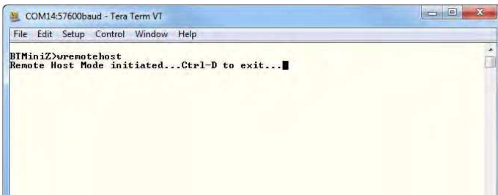
Figure 16. wRedirect Command Screen
