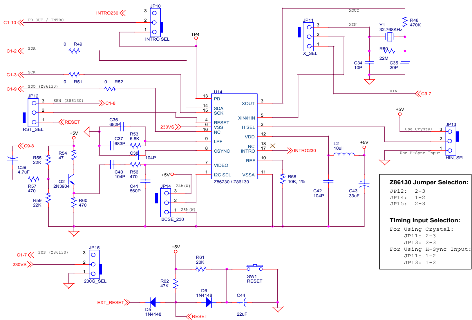
Figure 14. Z86130/230 Module Schematic
