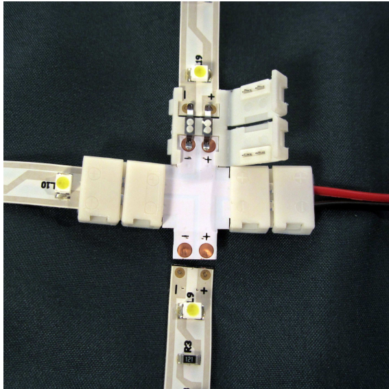
PRODUCT ASSEMBLED
