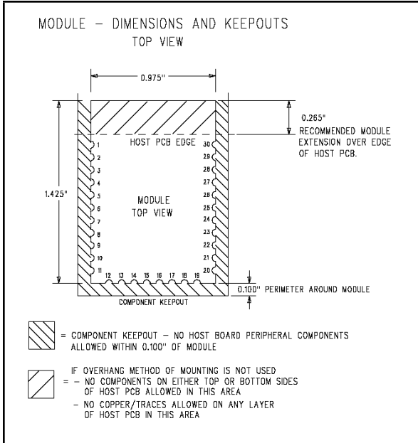
Module - Dimensions and Keepouts
