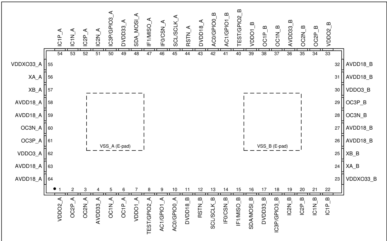
Figure 3 - Pin Diagram
