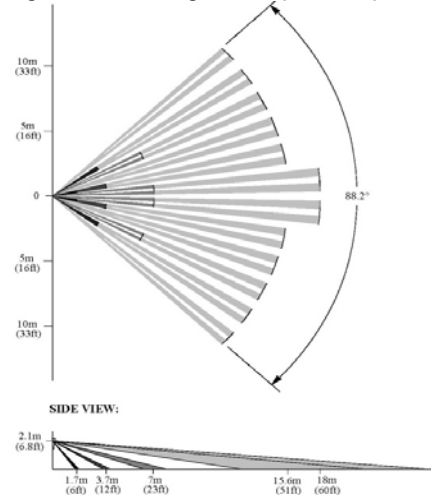
Figure 1. Wide Angle Lens (Installed)
