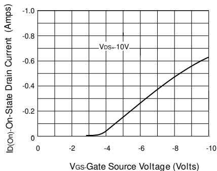
Transfer Characteristics
