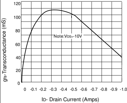
Transconductance v drain current
