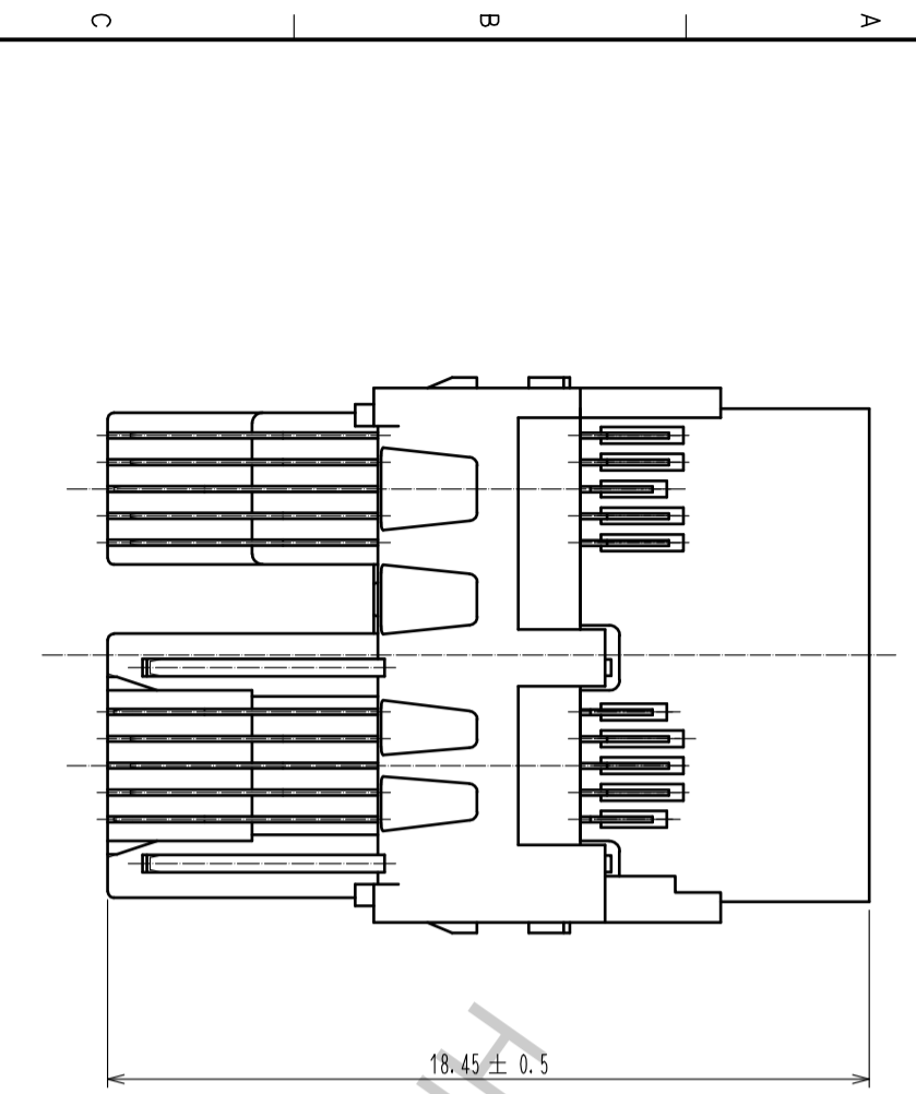
Fig-2. CONNECTOR MOUNTED ON PCB
