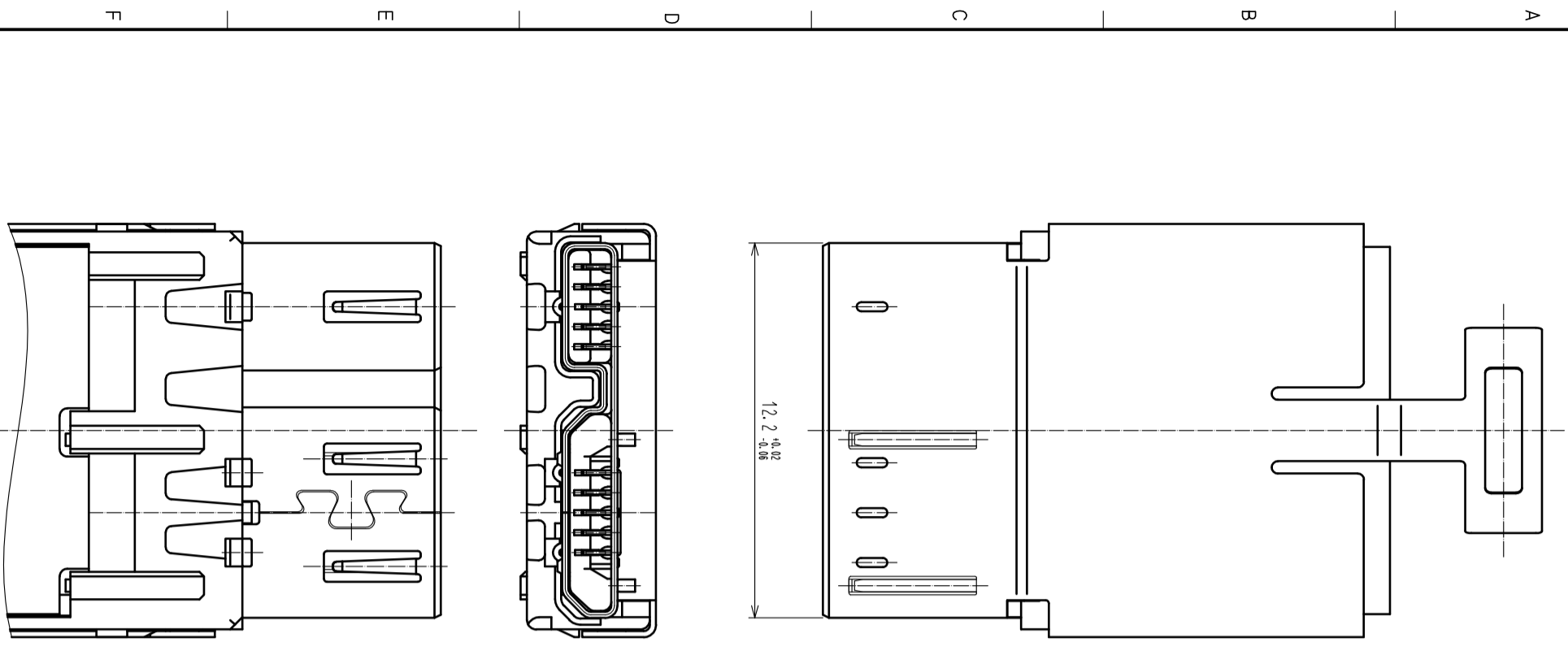
Fig-3 SHIELDING-PLATE ASSEMBLY
