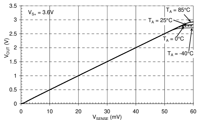
Output Voltage vs. Sense Voltage
