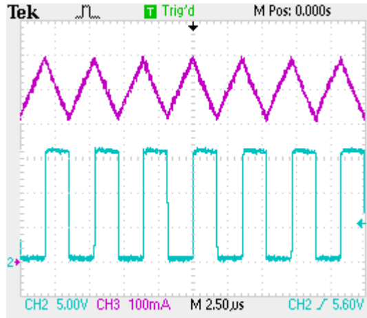
Actual Operating Waveforms [ V_{IN} = 30V , R_S = 0.36V , L = 68\mu H ] Normal operation. Output current (Ch3) and LX voltage (Ch2)
