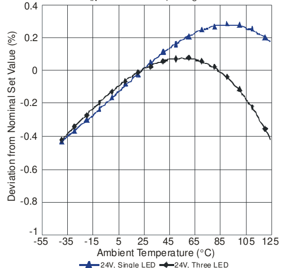
Output Current Change vs. Temperature
