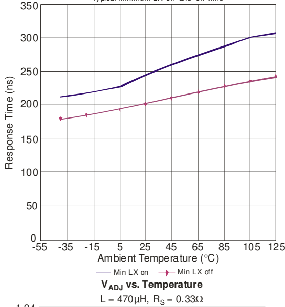
ZXLD1360 Response Time vs. Temperature Typical minimum LX 'on' and 'off' time
