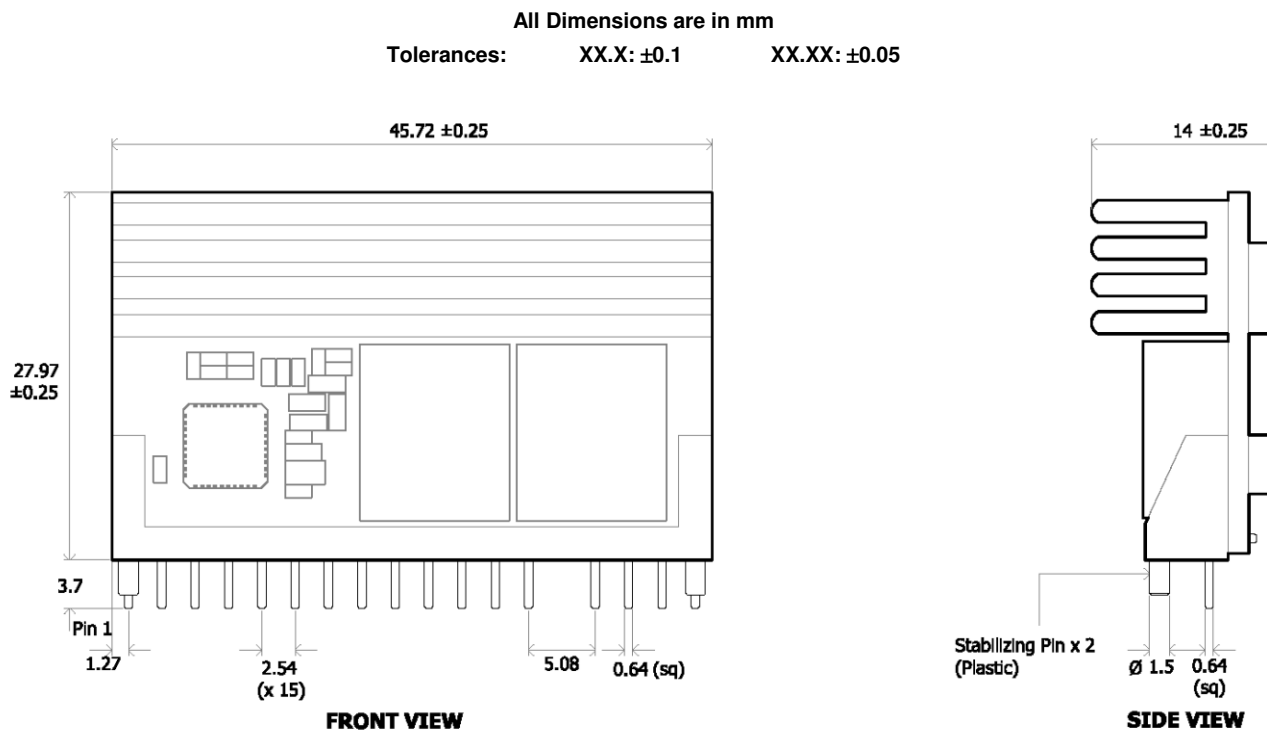
Figure 14. Mechanical Drawing
