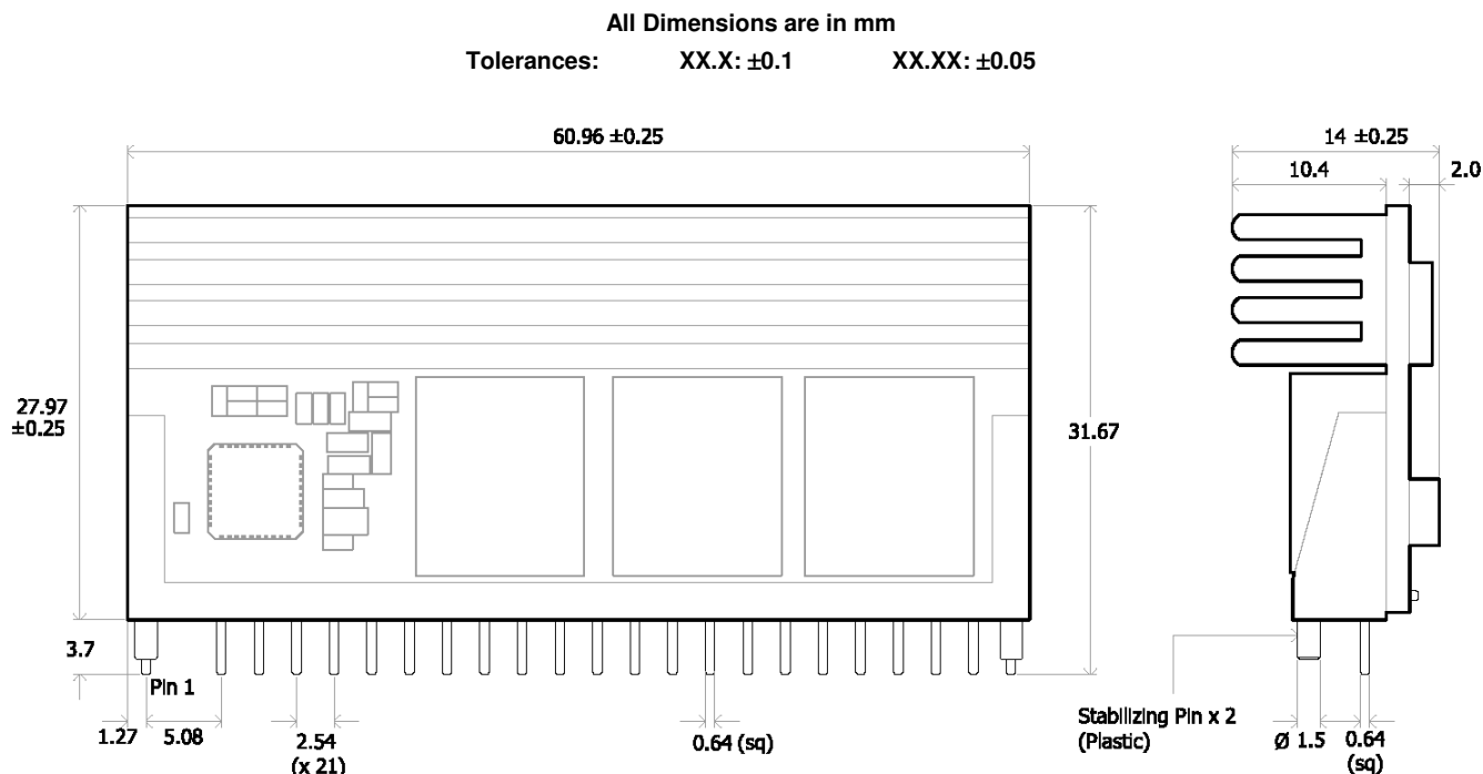
Figure 14. Mechanical Drawing
